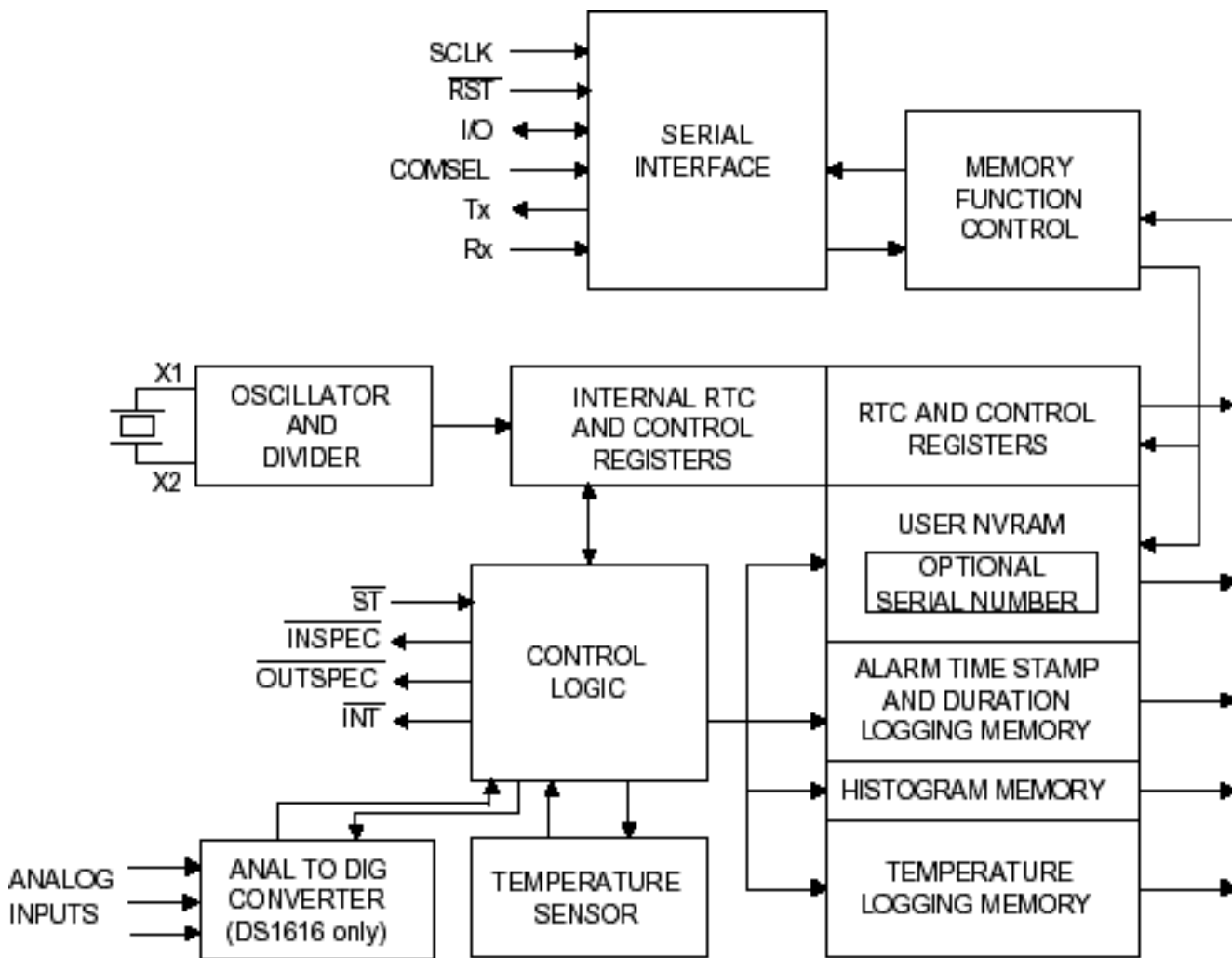
Figure 1. DS1615 Block Diagram
