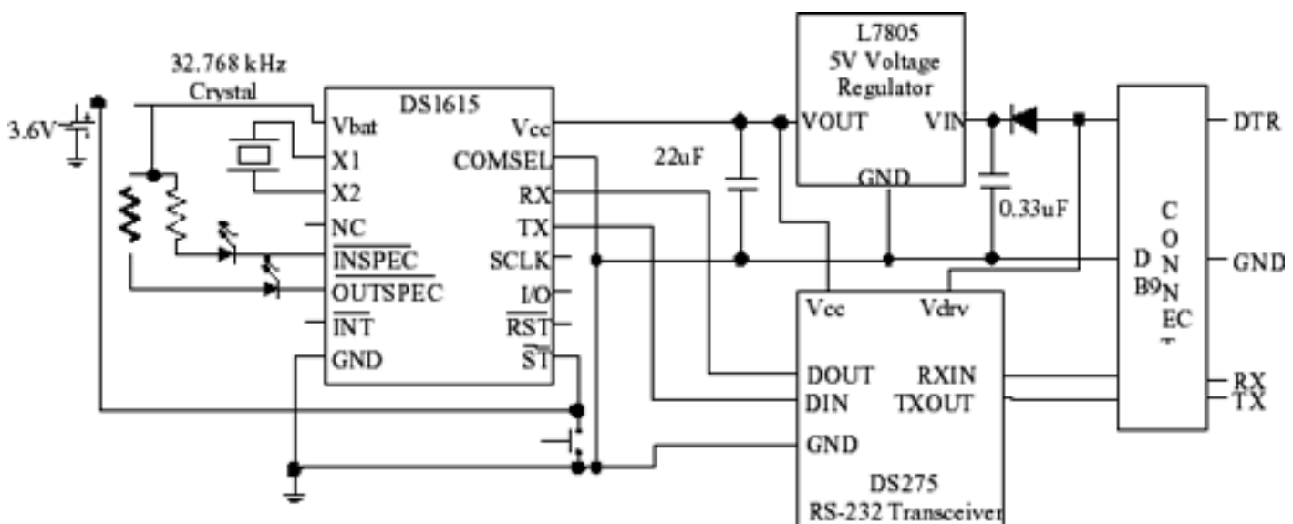
Figure 2. DS1615 as a Portable Datalogger
