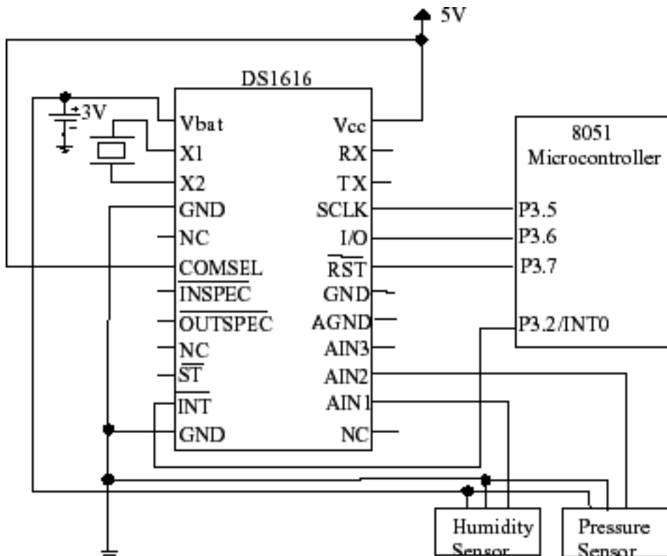
Figure 3. DS1616 in Embedded System
